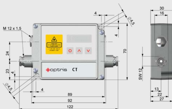
Electronics
