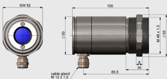
Sensing head
